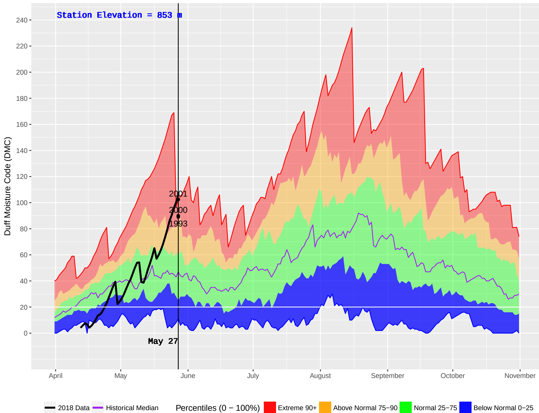
JOHNSON LAKE (419) : Historical (1986–2016) and Current (2018) Noon Duff Moisture Code (DMC)
