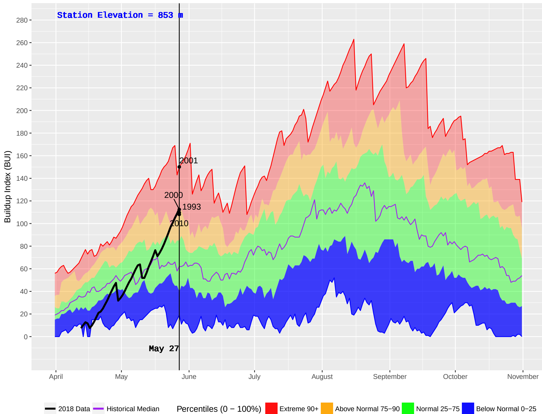
JOHNSON LAKE (419) : Historical (1986–2016) and Current (2018) Noon Buildup Index (BUI)
